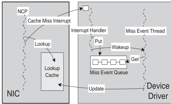
Figure 2: Cache miss handling path.
