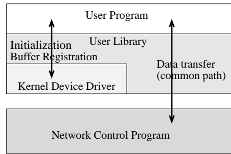
Figure 1: The general architecture of user-level communication systems.
