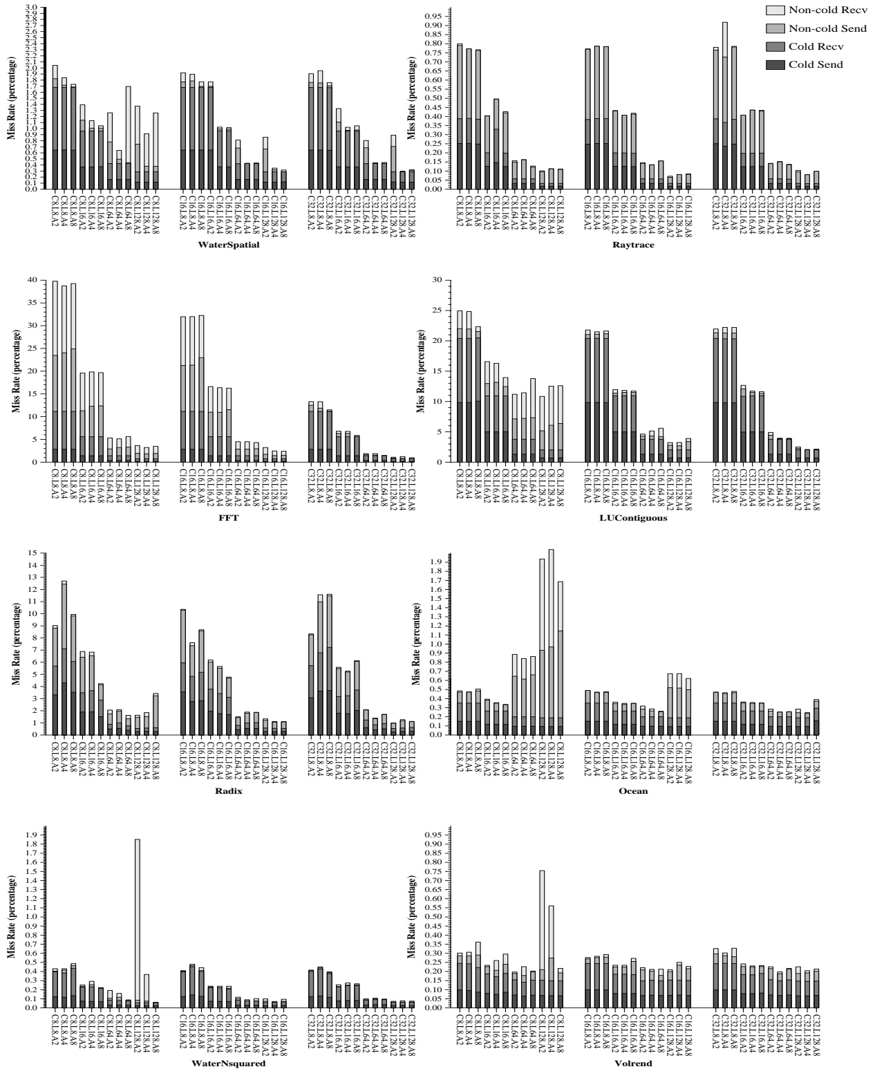
Figure 7: VMH lookup cache miss breakdown of the SPLASH-2 applications.
