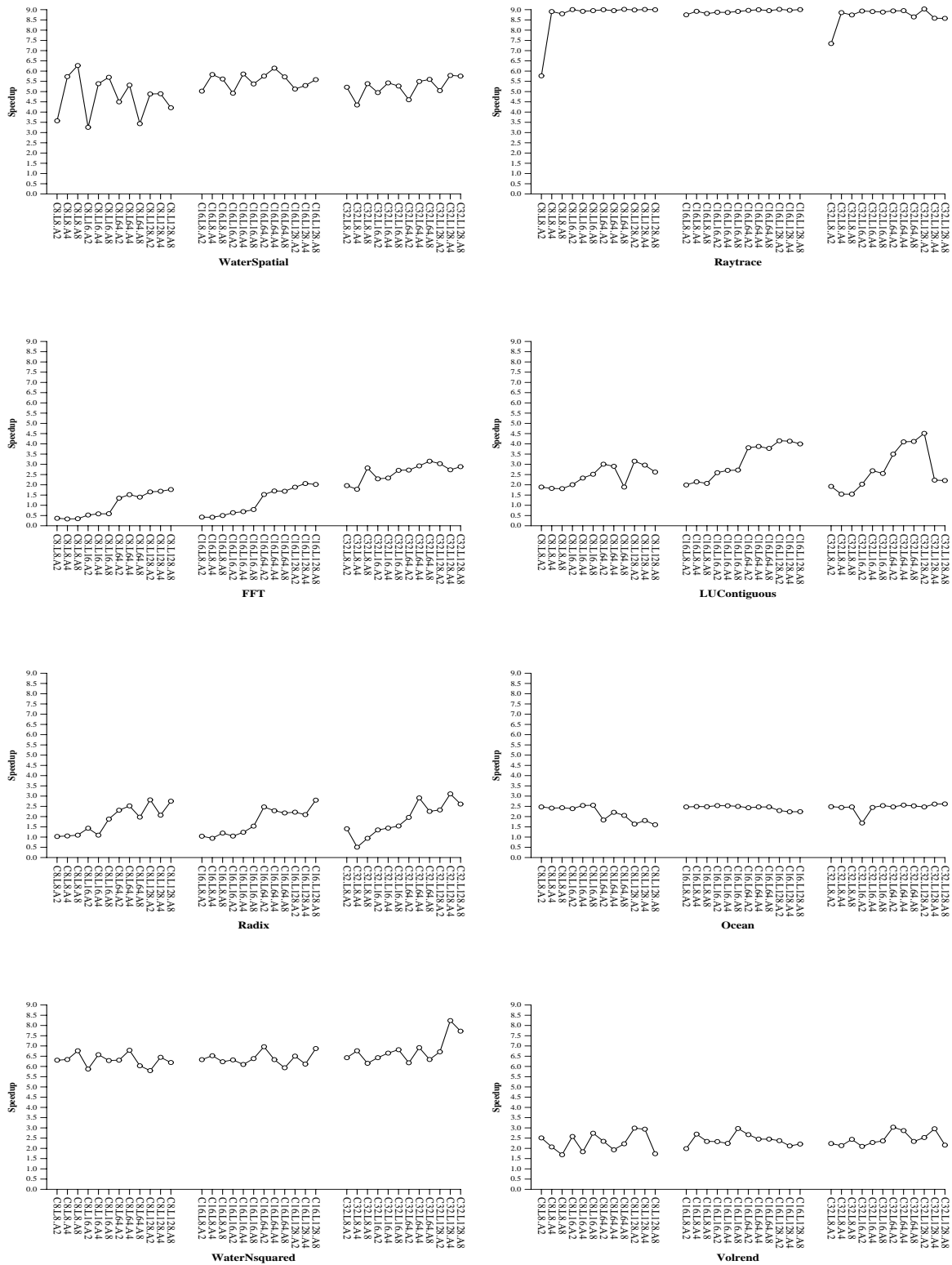
Figure 8: Parallel speedup of the SPLASH-2 applications in different VMH lookup cache configurations (8 processors used).
