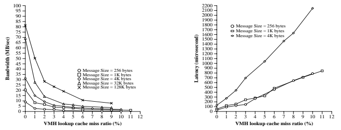
Figure 5: Effect of VMH miss on ping-pong latency and bandwidth.
