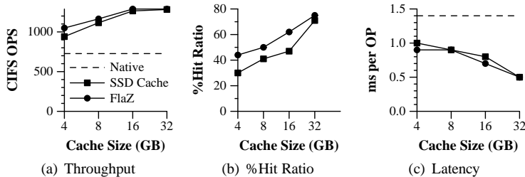
Figure 6. SPECsfs results for the 8D-2S configuration.
