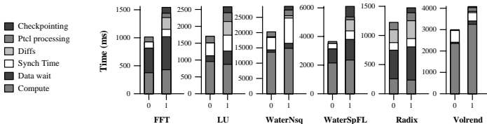
Figure 8. Overhead breakdown: 8 nodes, 1 thread/node.
