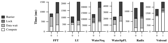
Figure 9. Execution breakdown: 8 nodes, 2 threads/node.
