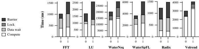
Figure 7. Execution breakdown: 8 nodes, 1 thread/node.
