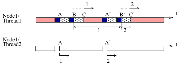
Figure 6. Recovery of failed threads.
