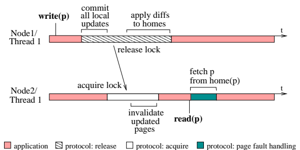
Figure 1. Basic SVM protocol operations.
