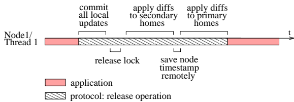
Figure 2. Diff propagation in the extended protocol.
