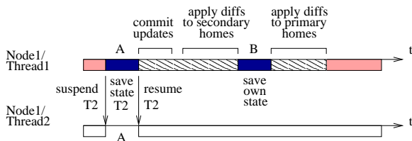
Figure 5. Thread state checkpointing.
