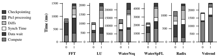
Figure 10. Overhead breakdown: 8 nodes, 2 threads/node.
